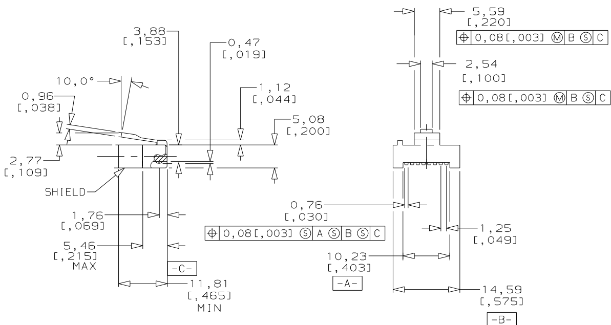
Figure 34 – Style-2 plug
