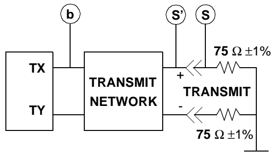
Figure 32 – Balanced transmitter test circuit
