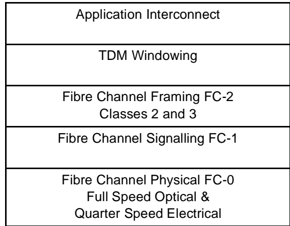
Figure 113 – Real Time Protocol Stack
