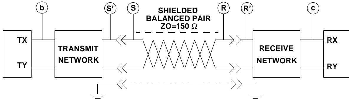
Figure 31 – FC-0 with 150Ω balanced cable link
