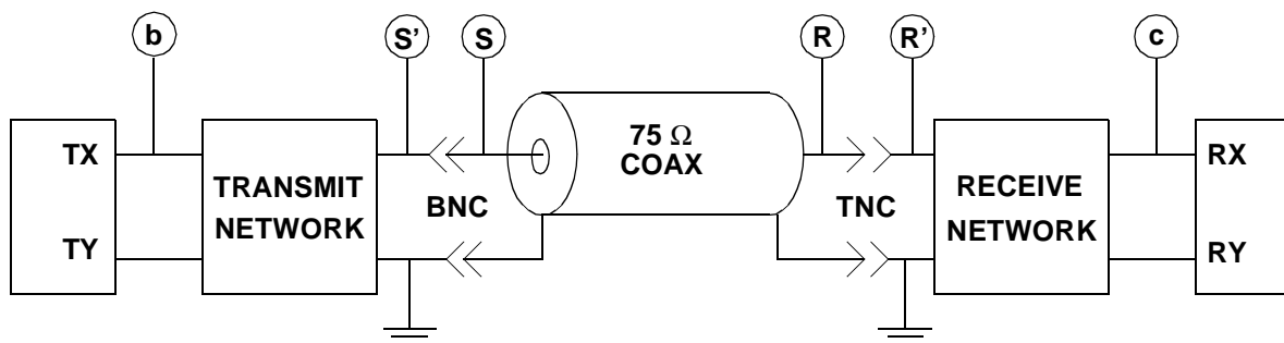
Figure 27 – FC-0 with 75Ω unbalanced cable
