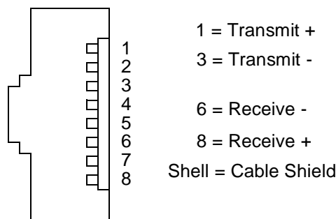
Figure 36 – Style-2 balanced connector receptacle pin locations
