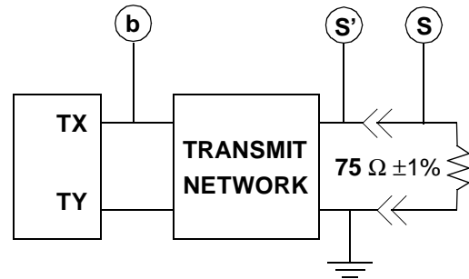
Figure 28 – Unbalanced transmitter test circuit
