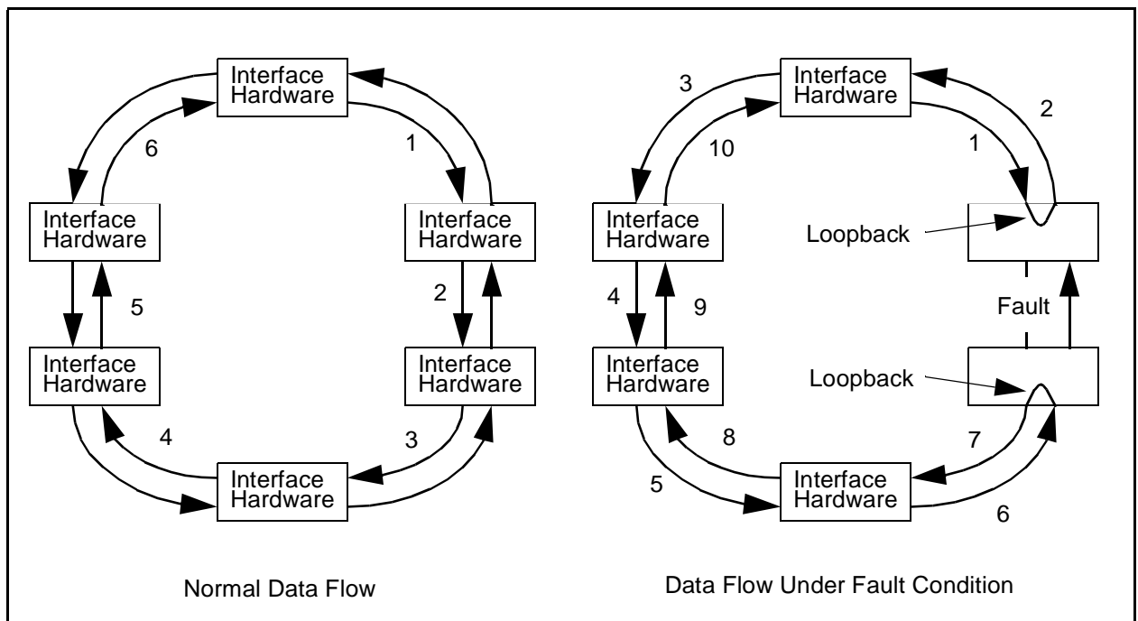
Figure 114 – Failure Detect and Re-routing
