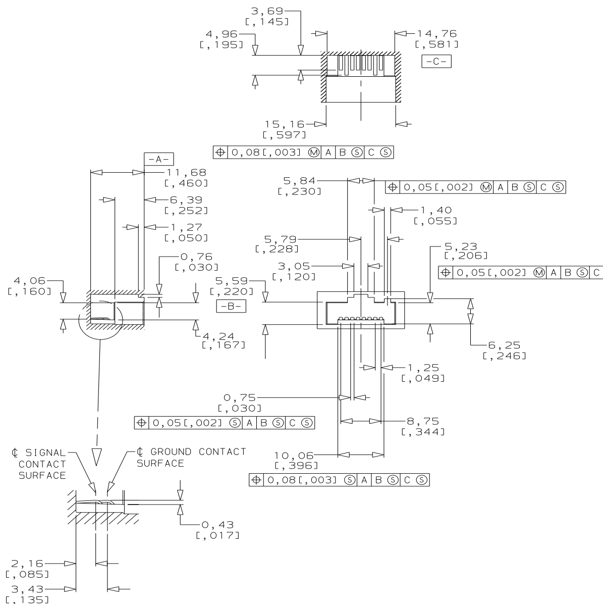
Figure 35 – Style-2 receptacle
