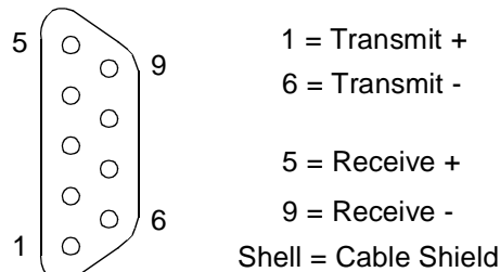
Figure 33 – Style-1 balanced connector pin assignments
