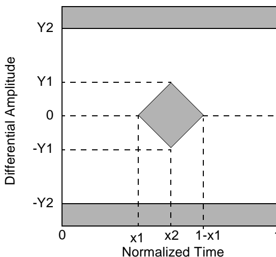
Figure 30 – Eye diagram mask at point-R'
