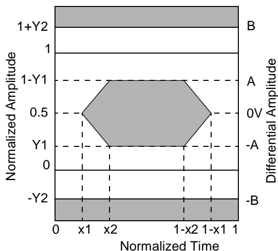
Figure 29 – Eye diagram mask at point-S
